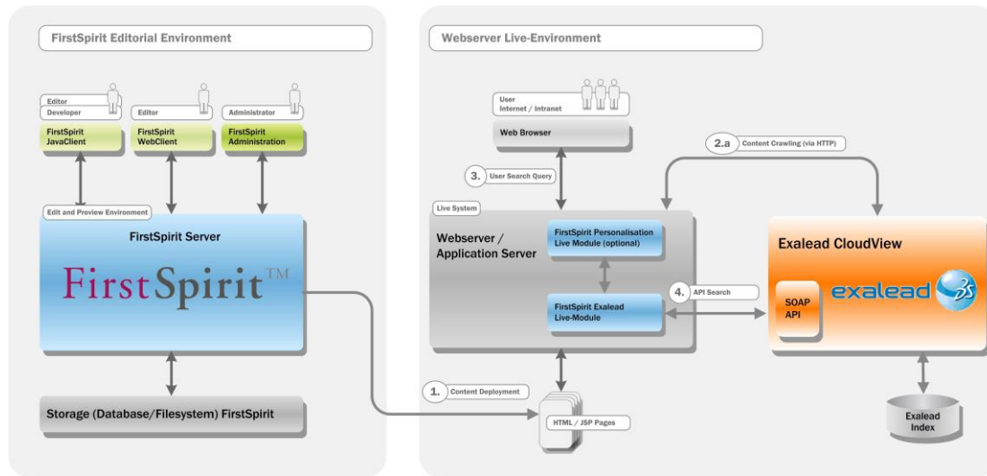
Figure 2-2: Personalized search
