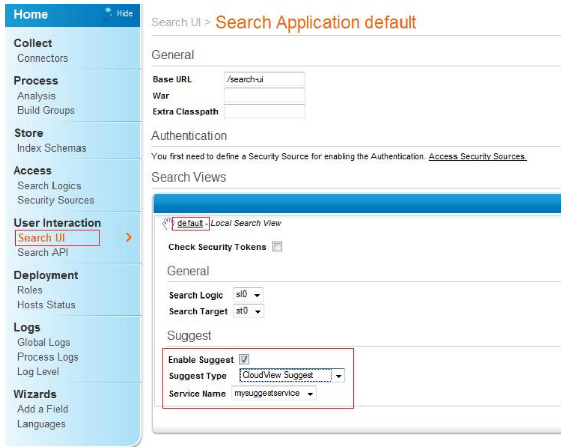
Figure 6-5: Activating the SuggestService
