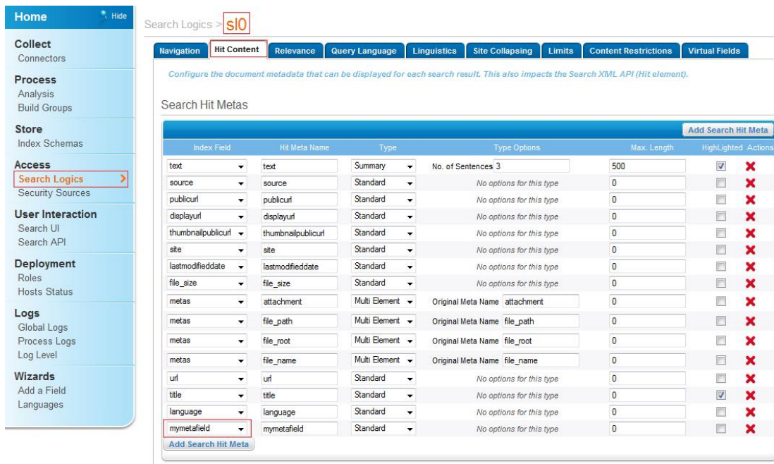
Figure 5-9 Adding a mapping target
