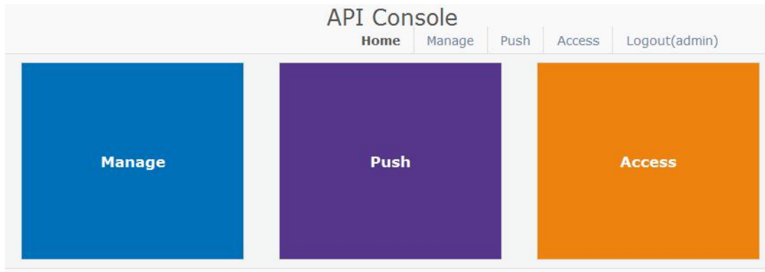
Figure 5-2 API Console
