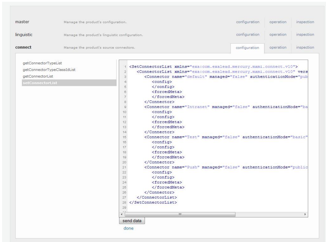
Figure 5-3 setConnectorList
