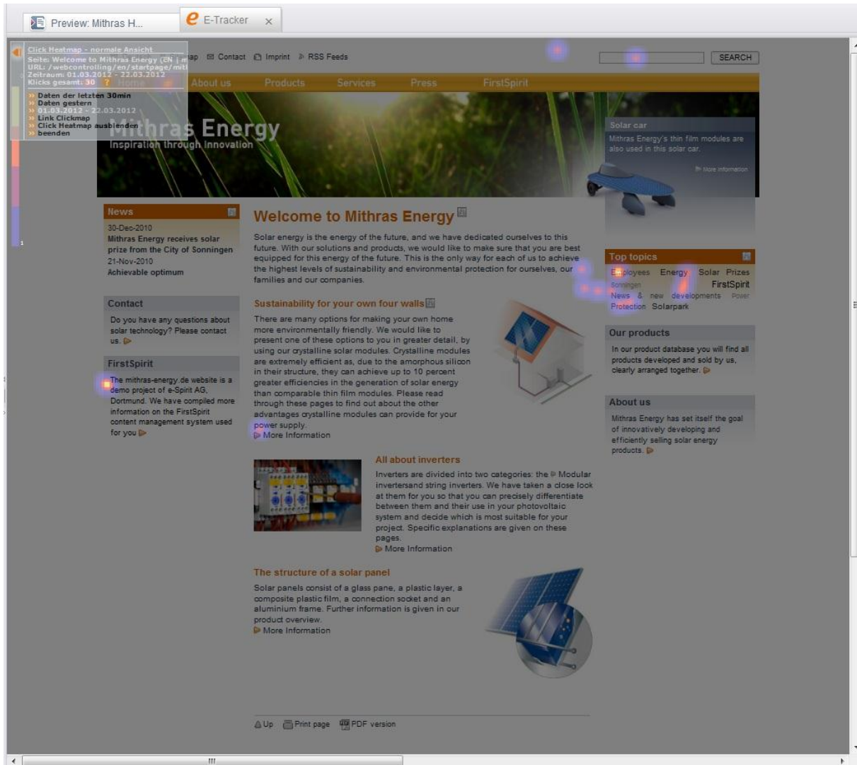
Figure 4-5 E-Tracker display from the "Show Heatmap" script
