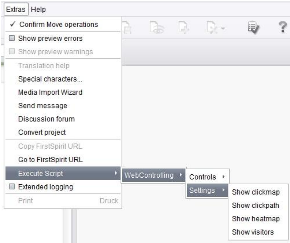
Figure 3-1 Selection of the scripts via the menu
