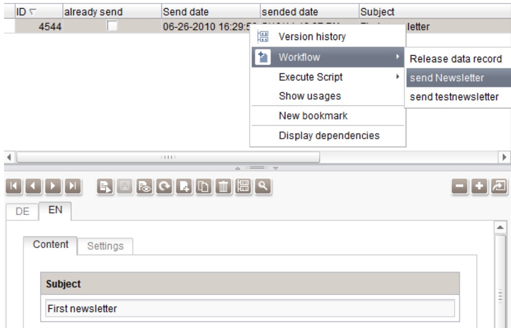
Figure 7-3: Starting workflow
