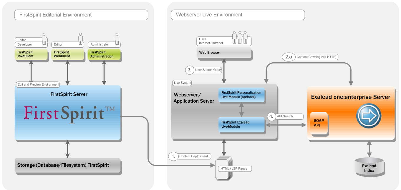
Figure 2-2: Personalised search
