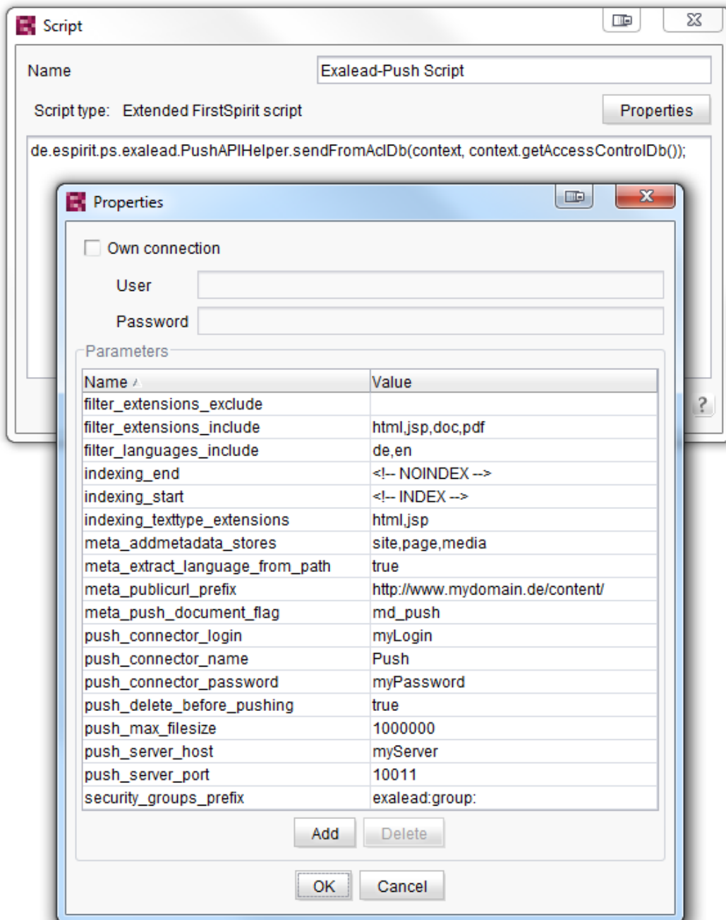
Figure 6-2: Script properties
