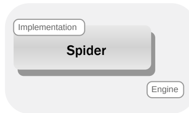
Figure 2-2: Engine implementations
