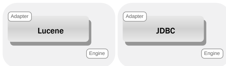
Figure 2-3: Engine adapters
