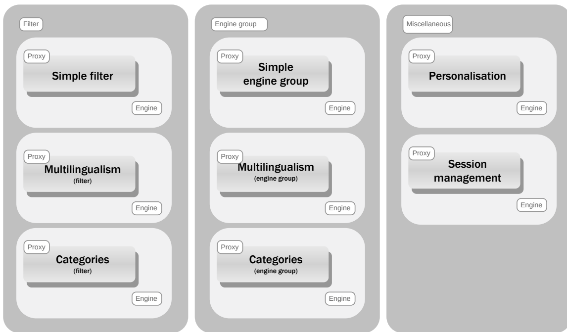
Figure 2-5: Engine proxies
