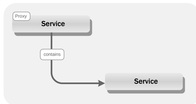
Figure 2-8: Service proxy
