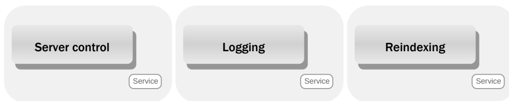
Figure 2-7: Services
