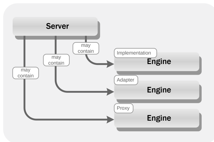
Figure 2-6: Server
